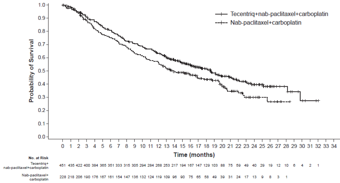
Figure 6: Kaplan-Meier curves for overall survival (IMpower130)
