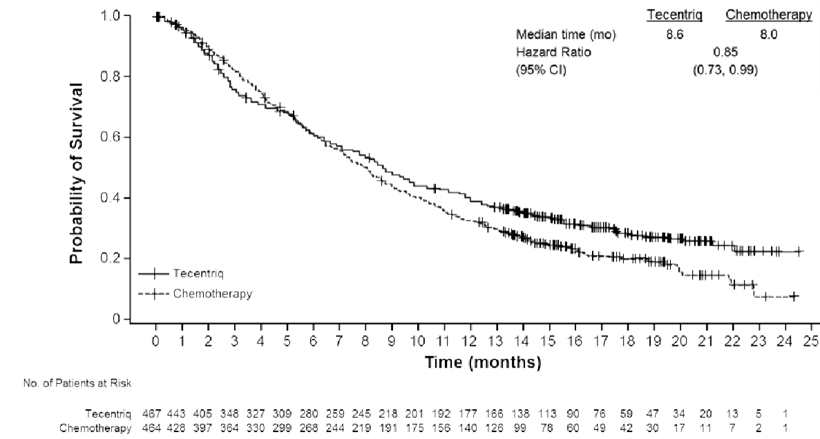
Figure 1: Kaplan-Meier curve for overall survival (IMvigor211)
