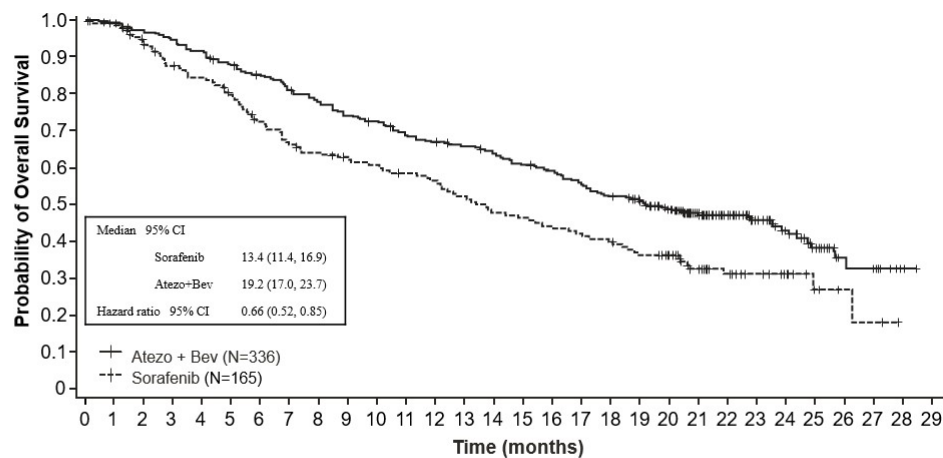
Figure 18: Kaplan-Meier curve for OS in the ITT population (IMbrave150 Updated Analysis)
