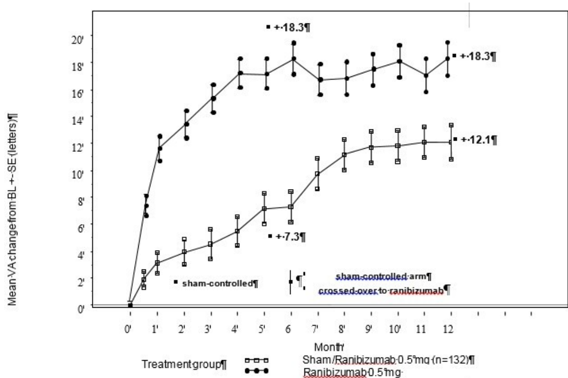
Figure 12-4 Mean change from baseline BCVA over time to Month 6 and Month 12 (BRAVO)
