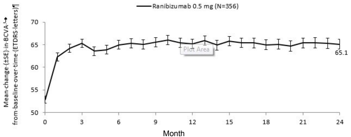
Figure 12-7 CRYSTAL: Mean change in BCVA from baseline over 24 months
